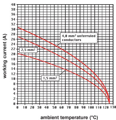
CQY..E 8 poles connector inserts Maximum current load derating diagram
